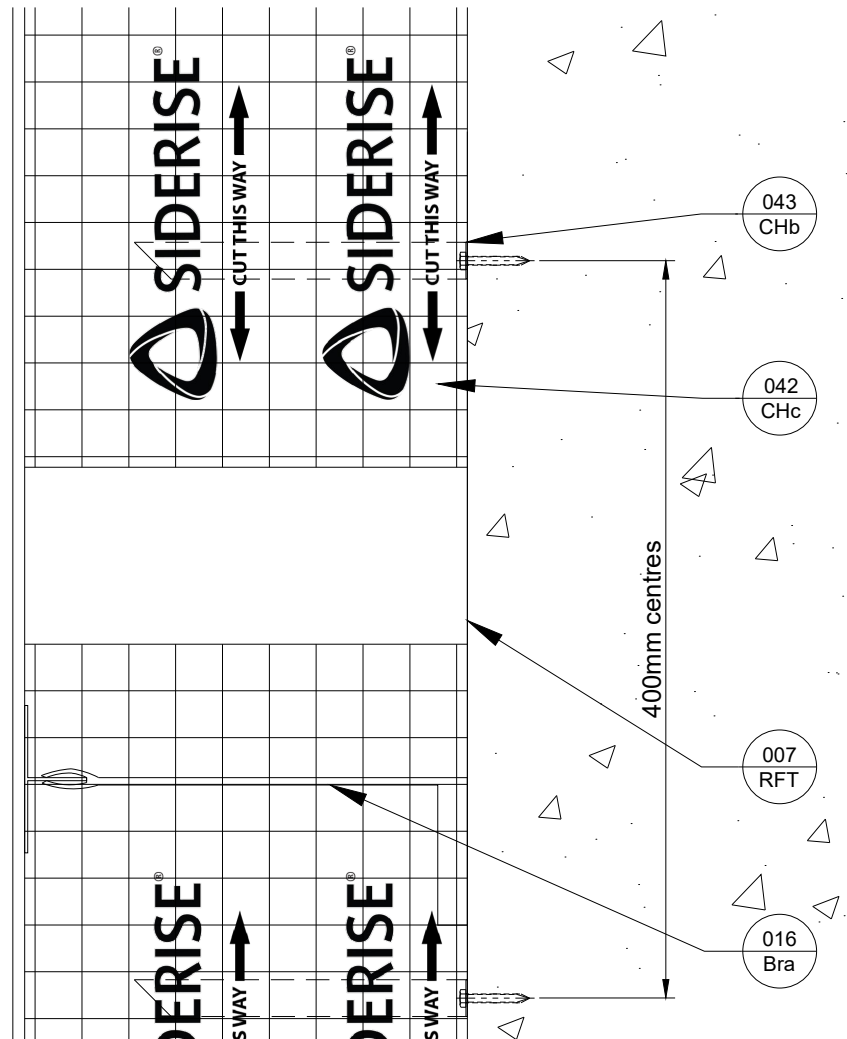
Plan View
