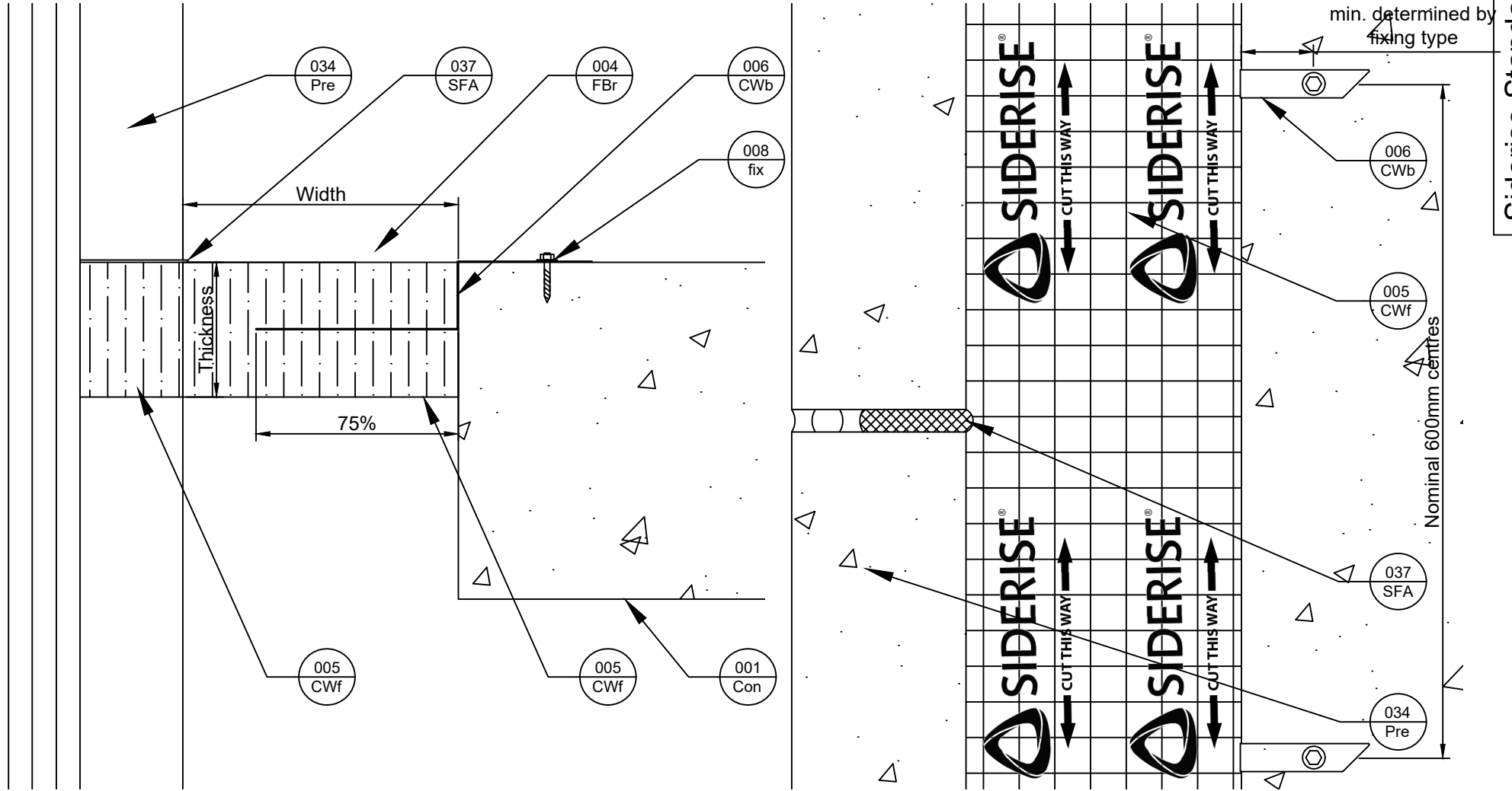
Side View
