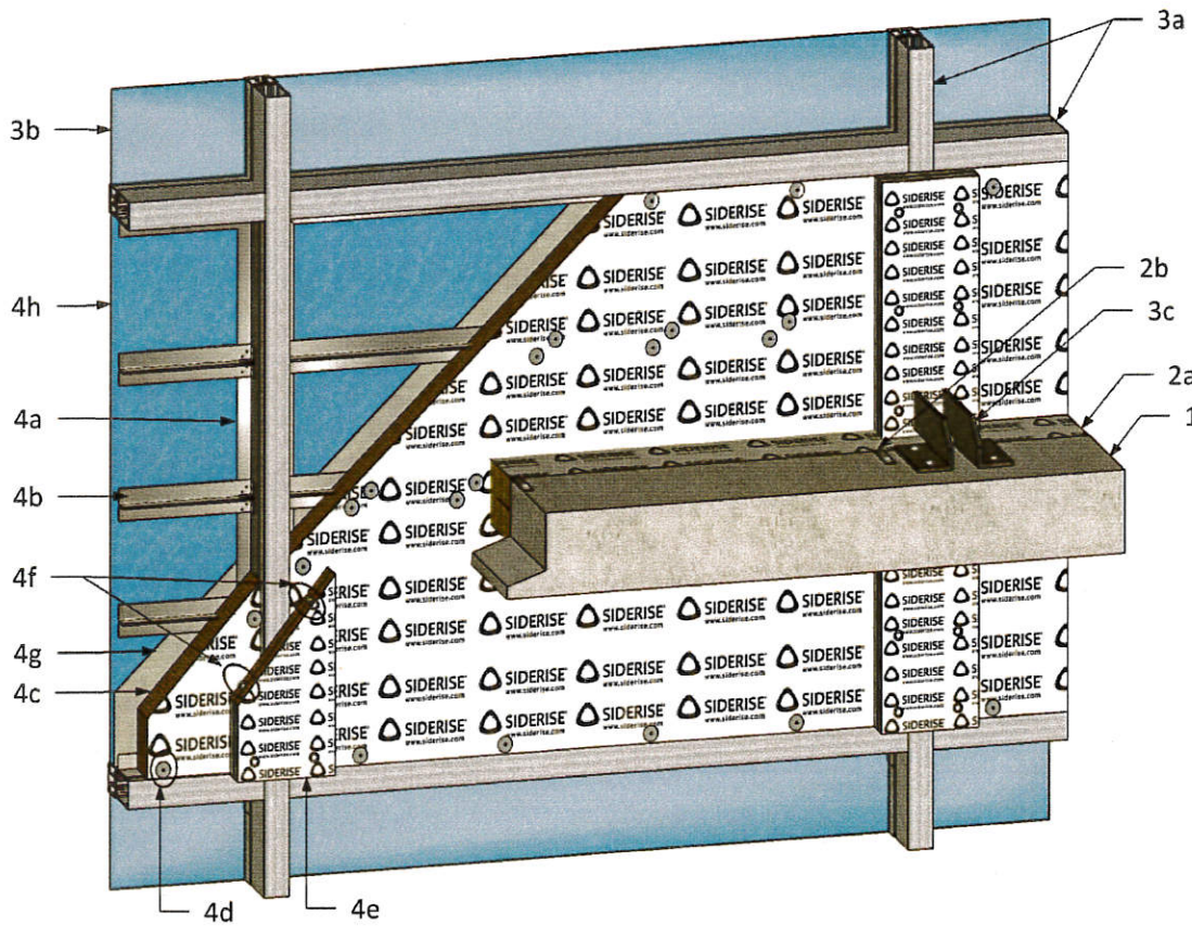
Figure 1: System details – spandrel area
