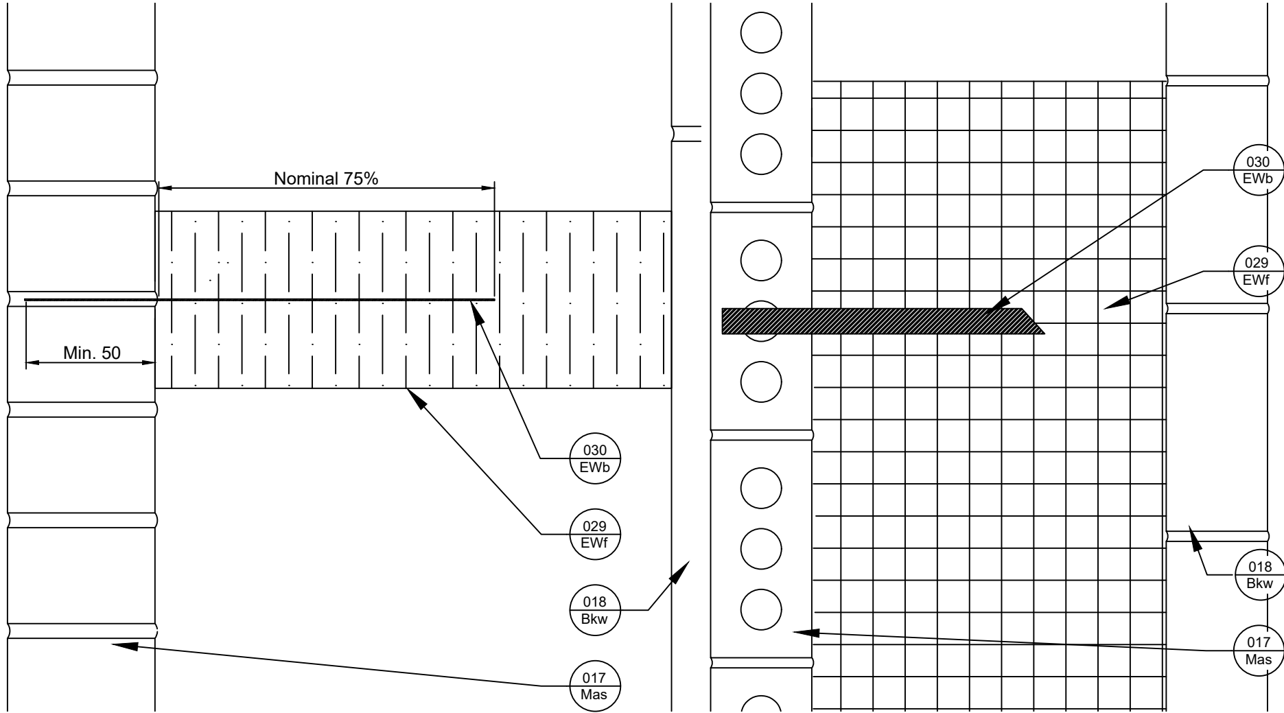
Side View
