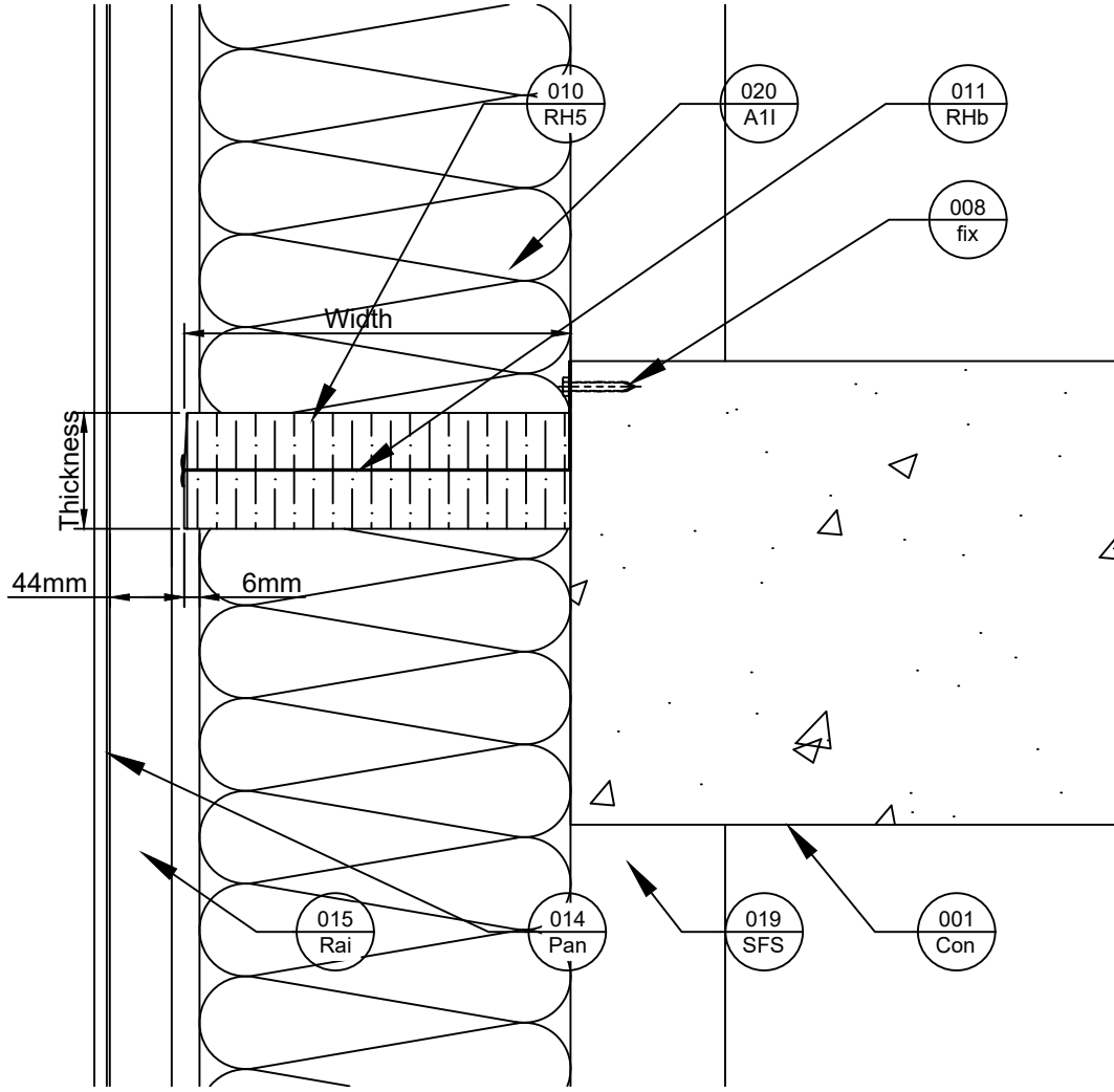
Side View
