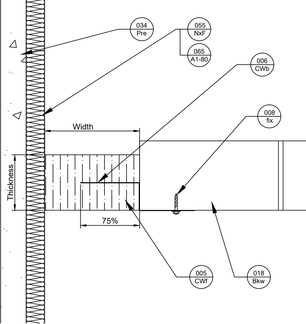
Plan View
