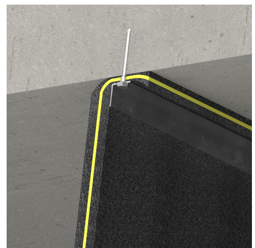
Fig 2. Head Fixing
