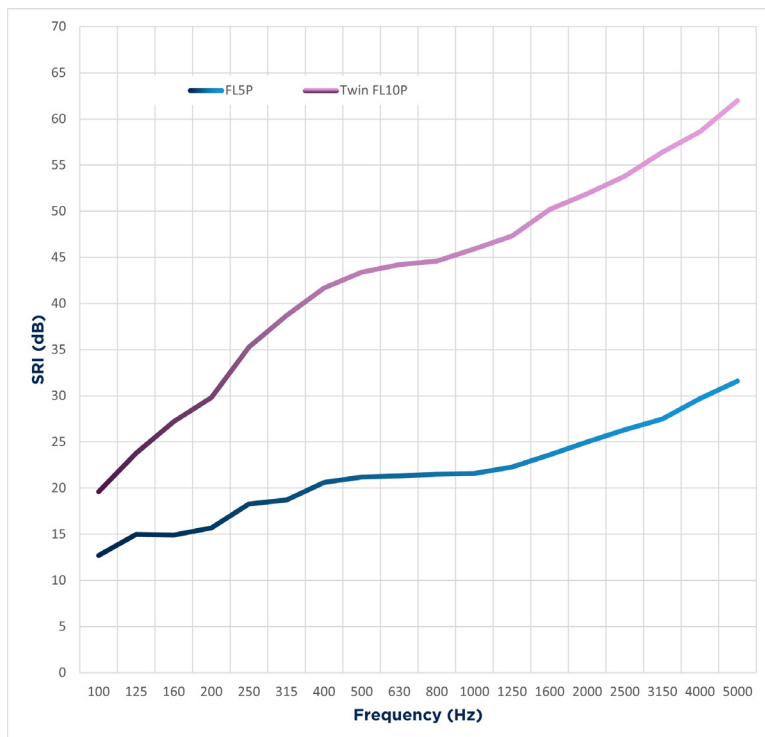
Graph 1 - 1/3 rd Octave Data for FL5P & Twin FL10P
