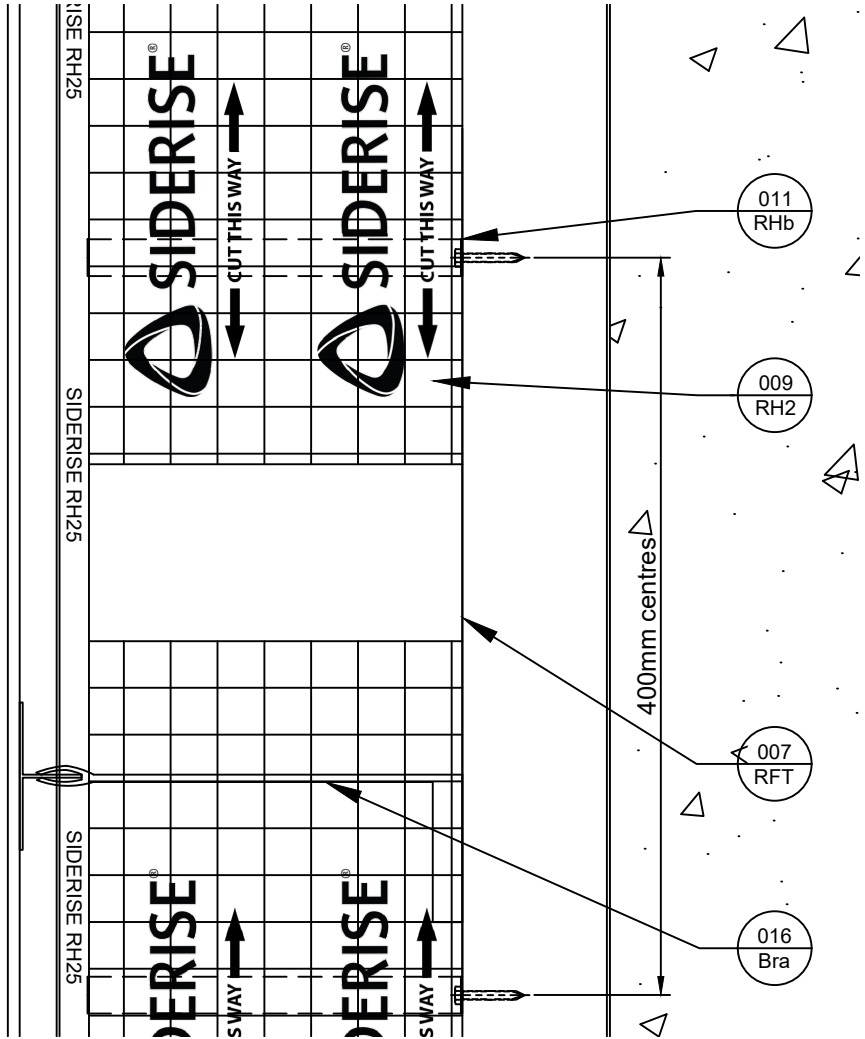
Plan View
