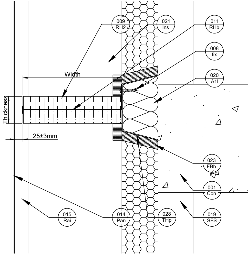
Side View
