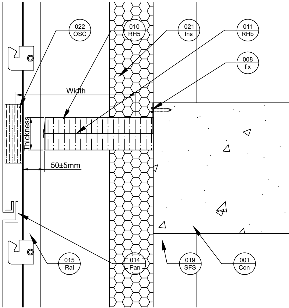
Side View
