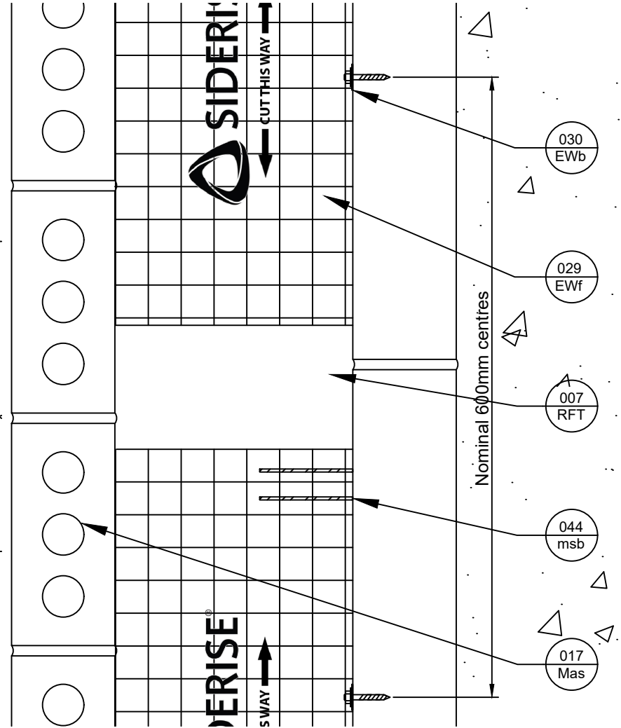
Plan View
