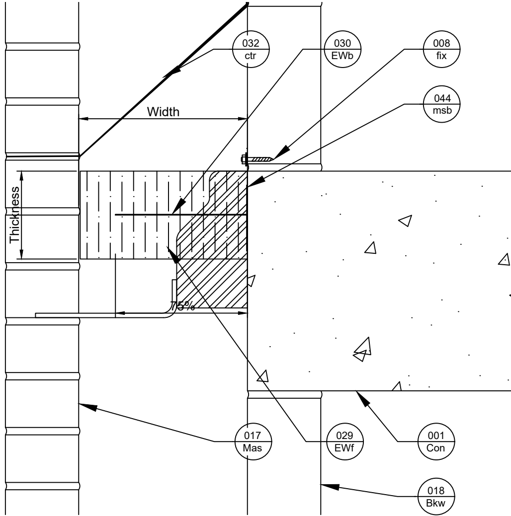
Side View
