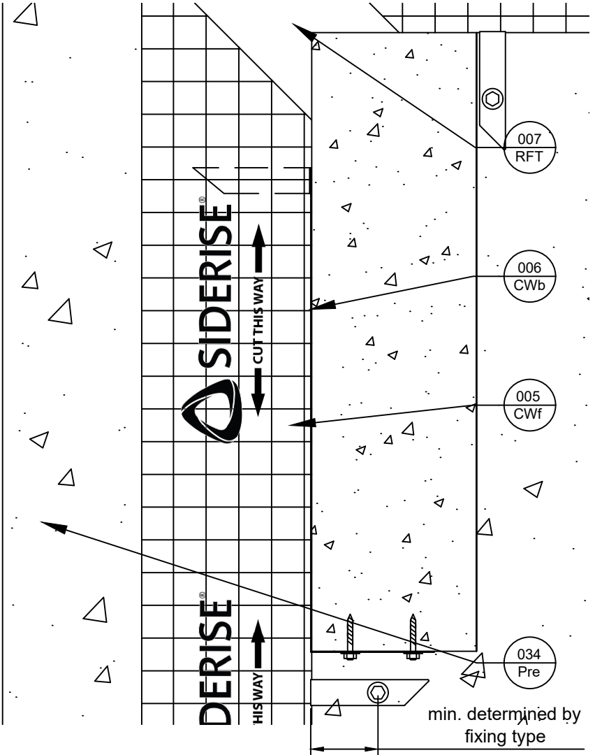
Plan View
