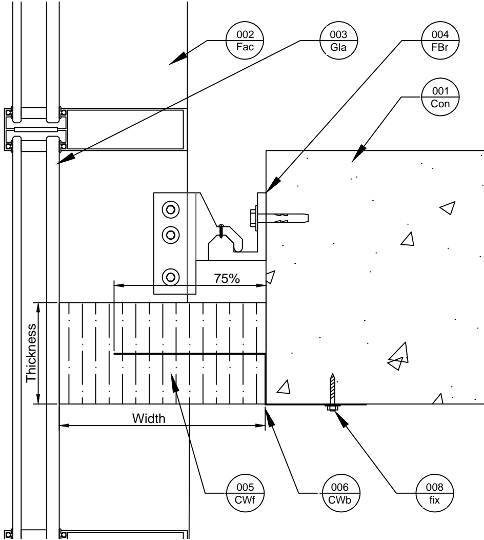
Side View
